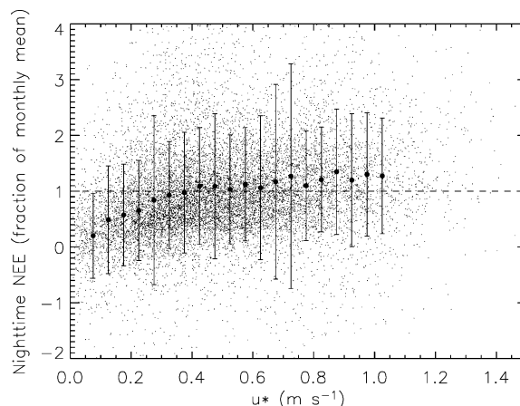
Fig. 3. Normalized nighttime NEE as a function of u_* at the Willow Creek tower (long-term data from 1999 to 2002, excluding wind directions from that were associated with venting anomalies). Solid circles with error bars represent means and standard deviations of data binned by u_* in increments of 0.05 \text{ m s}^{-1} .
