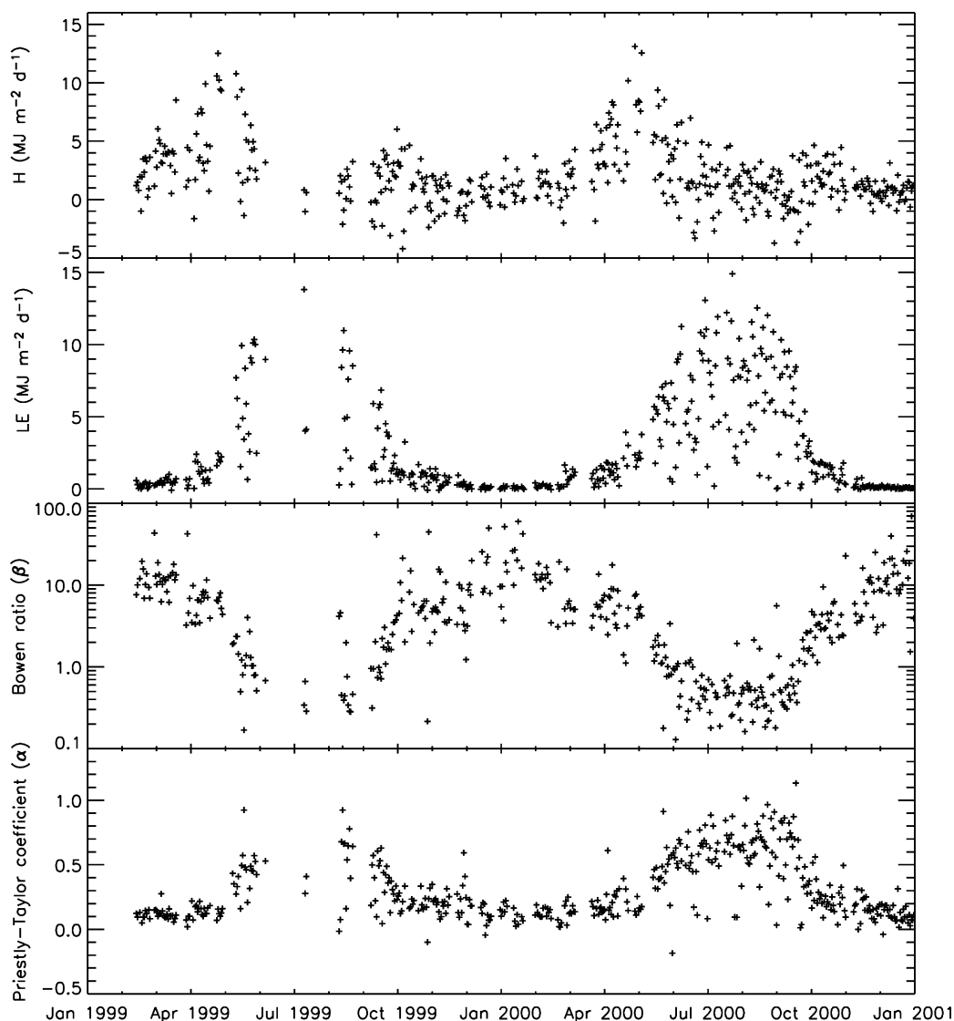
Fig. 13. Seasonal changes in daily integrated (a) sensible and (b) latent heat fluxes; (c) integrated midday (1000–1400 CST) Bowen ratio; (d) the Priestly–Taylor constant, \alpha = ET_{\text{Actual}}/ET_{\text{eq}} , from the Willow Creek flux tower (1999–2000).
