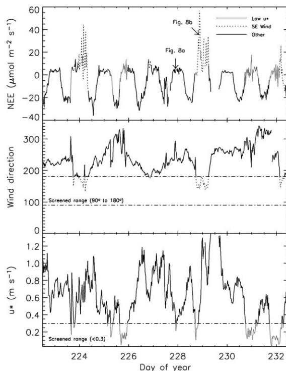
Fig. 7. Above-canopy NEE measurements and micrometeorological conditions at Willow Creek (August 9–20, 2002) that were used to screen data for weak turbulence ( u_* < 0.3 \text{ m s}^{-1} ; gray line) and non-representative sampling conditions (SE winds; dotted line). Nighttime and early morning venting anomalies from the SE quadrant were not associated with weak turbulence; venting events lasted several hours; and elevated fluxes during venting could be differentiated from random signal noise associated with weak turbulence.
