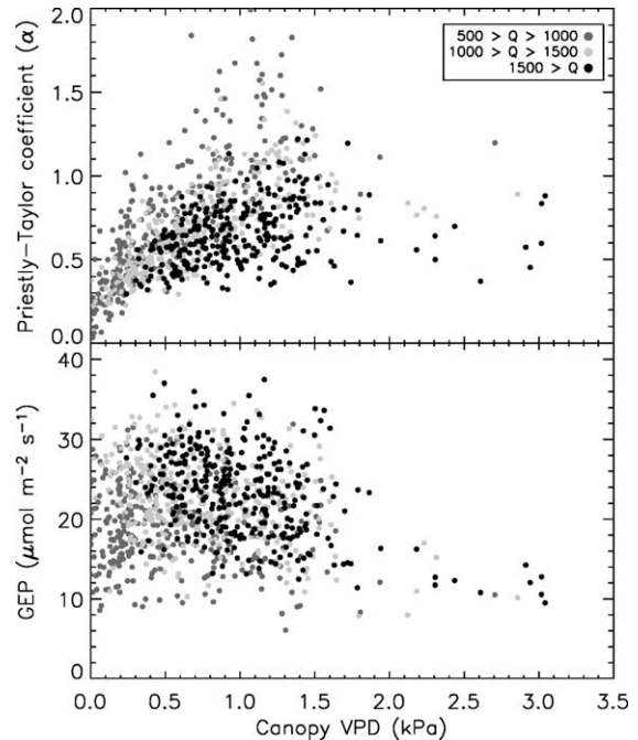
Fig. 14. Influence of half-hourly vapor pressure deficits (VPD) and incoming radiation on (a) relative evapotranspiration and (b) gross ecosystem production (GEP) observed from the Willow Creek flux tower during 2000. Symbol color indicates level of photosynthetically active radiation ( Q ): medium gray, 500\text{--}1000 \mu\text{mol m}^{-2} \text{ s}^{-1} ; light gray, 1000\text{--}1500 \mu\text{mol m}^{-2} \text{ s}^{-1} ; black, >1500 \mu\text{mol m}^{-2} \text{ s}^{-1} . Data was screened for precipitation events and condensation to avoid the confounding effects of water on leaves and sensors.
