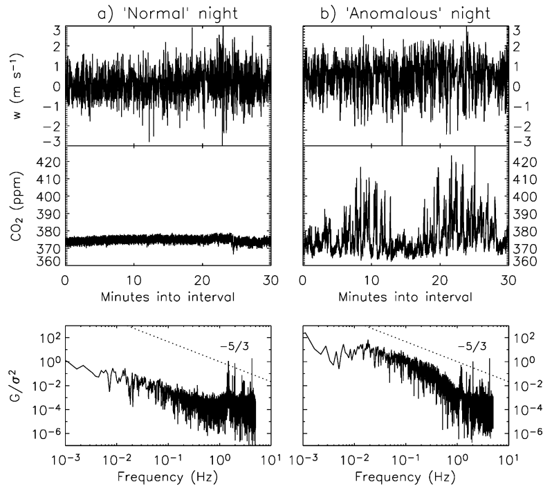
Fig. 8. Fast (10 Hz) time series of vertical velocity ( w ) and \text{CO}_2 mixing ratio, and normalized \text{CO}_2 spectra for sequential nights in August 2000 (see Fig. 7) during which (a) venting was not observed, and (b) venting was observed.
