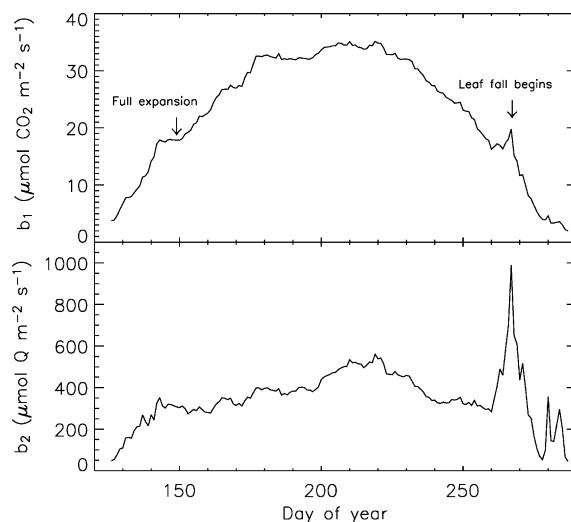
Fig. 10. Changes in photosynthesis model parameters, maximum assimilation rate ( b_1 ) and photon flux density required for half saturation ( b_2 ) for Willow Creek during 2000.
