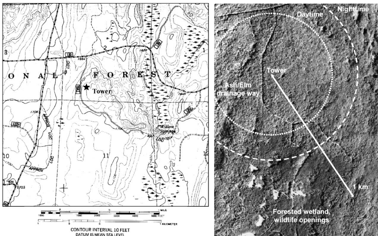
Fig. 1. (a) Local topography at the Willow Creek flux tower site (US Geological Survey, Pike Lake SE, Wisconsin, scale 1:24 000, series V861, sheet 1, US Government Printing Office, 1997); (b) estimated daytime and nighttime tower footprint ( u_* > 0.3 \text{ m s}^{-1} ) shown on a multi-spectral image of vegetation (ATLAS aircraft, 1998; bands 6, 7, 4). An arrow is used to indicate the wind vector associated with the largest nighttime and early morning venting anomalies.
