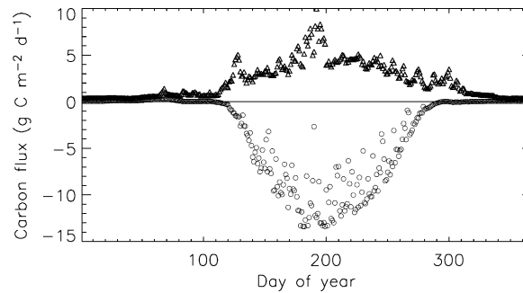
Fig. 12. Daily partitioning of NEE between gross photosynthesis (circle) and ecosystem respiration (triangle) at Willow Creek during the period between full canopy development and leaf senescence, 2000.
