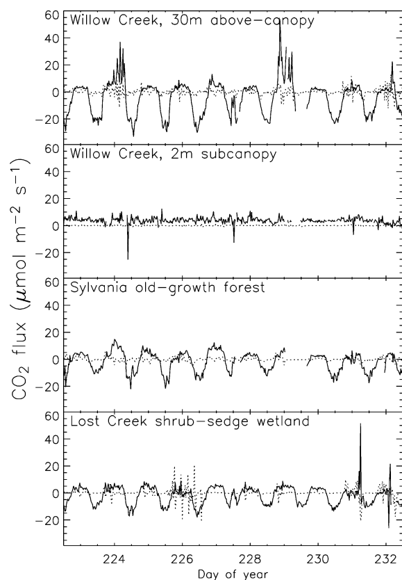
Fig. 6. Eddy covariance (solid line) and storage flux (dotted line) observations from four stations near the above-canopy tower at Willow Creek during August 9–20, 2002. Nighttime and early morning venting events on days 224 and 229 were unique to Willow Creek, and appeared only in the eddy covariance measurement above the forest canopy.
