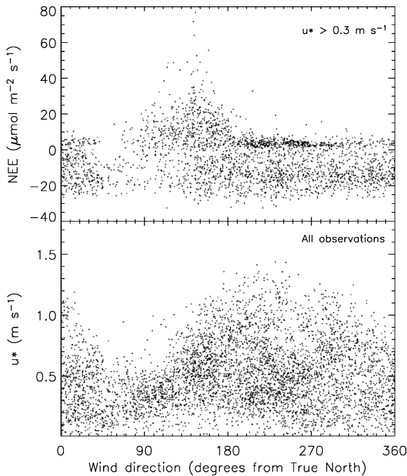
Fig. 4. Net ecosystem exchange (NEE) from 1999 and 2000 growing seasons, showing (a) exceptionally large respiration fluxes from the SE quadrant during valid turbulent conditions ( u_* > 0.3 \text{ m s}^{-1} ) and (b) reduced friction velocities ( u_* ) associated with local topography and higher elevations to the east.
